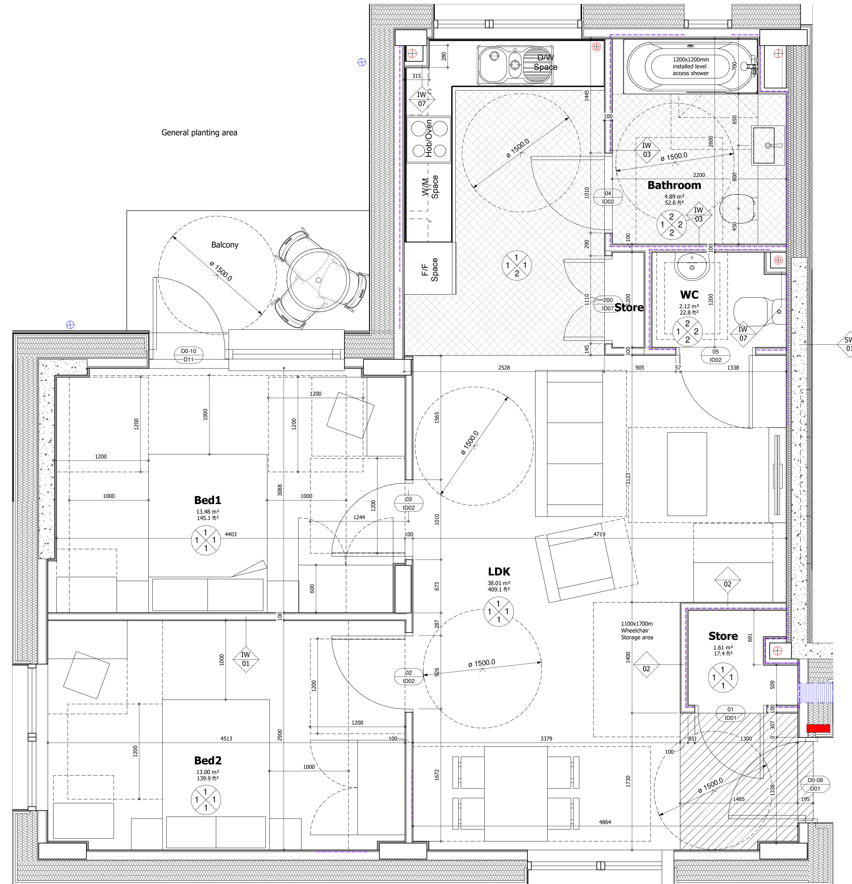
1 | Unit W.00.01 - Ground Floor 1:25
